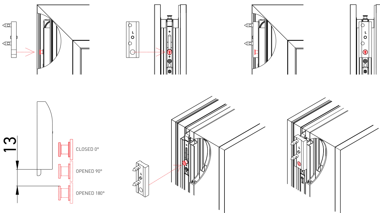
I7203-00-N03 Marking jig for locking plate
