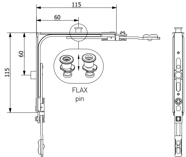
Corner transmission, bottom, 1FX +MAGNET
