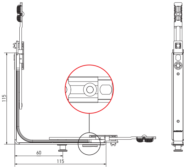
Corner transmission, bottom, 1 MR, 115×115
