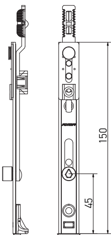
Bottom extension for turn sash 90° (bottom), 1 ML
