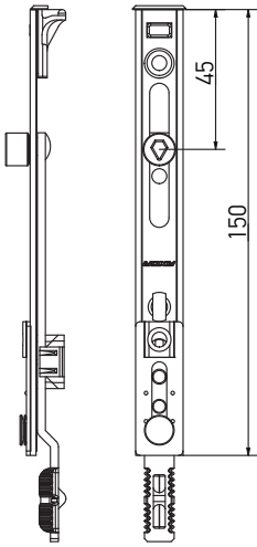
Bottom extension for turn sash 180° (top), 1 ML
