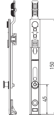
Bottom extension for turn sash 90° (bottom), 1 MR
