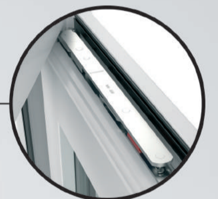
Stay arm Allows for the comfortable closing of the window due to the sash latch mechanism. Include blocking of the false handle turning in tilt mode
